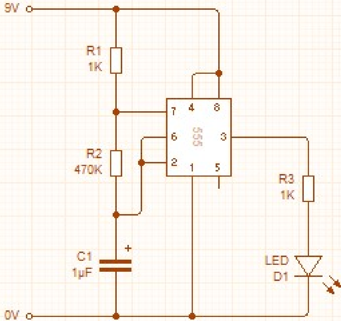
Flashing LED Schematic
