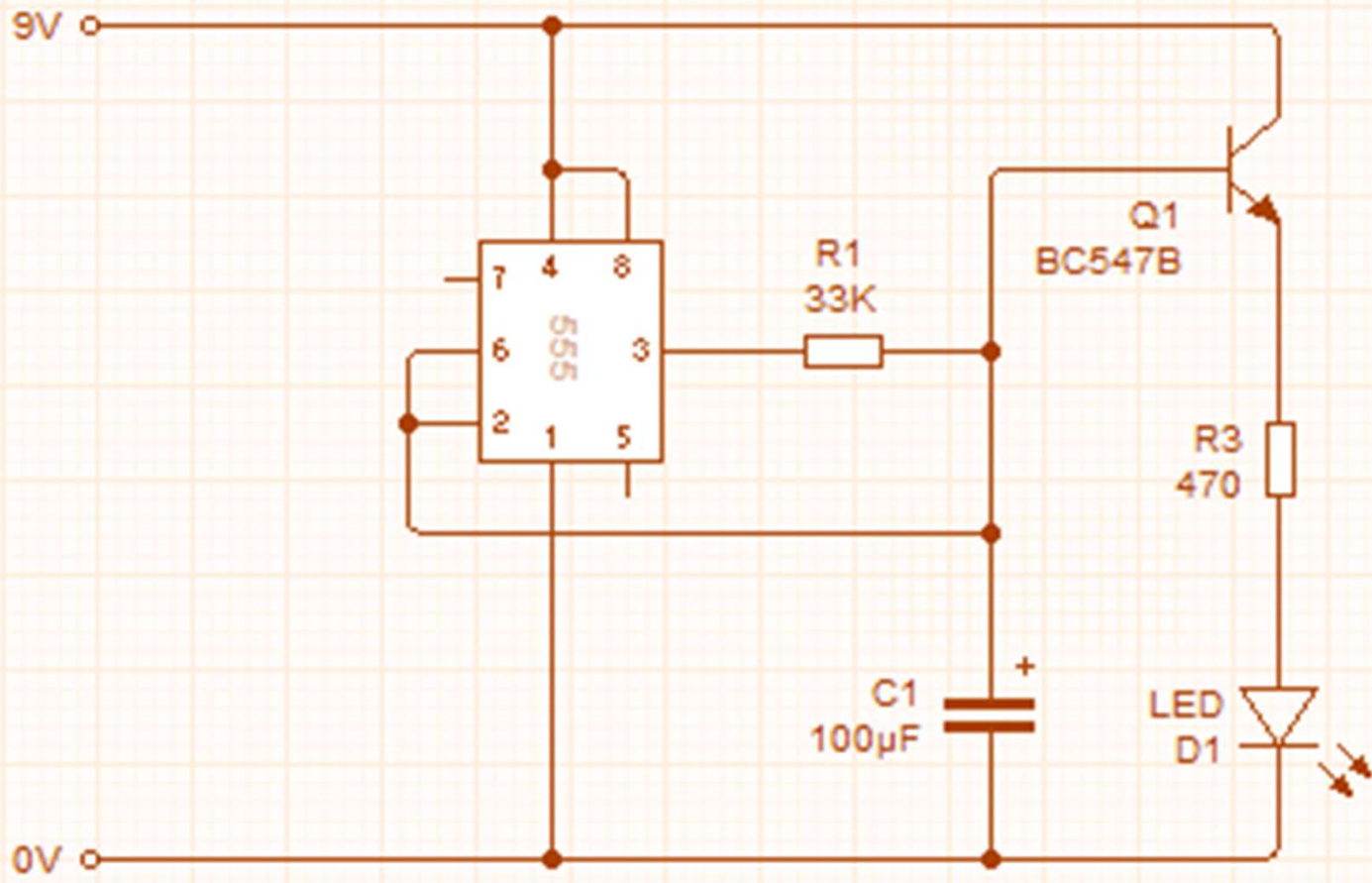
Fading LED Schematic
